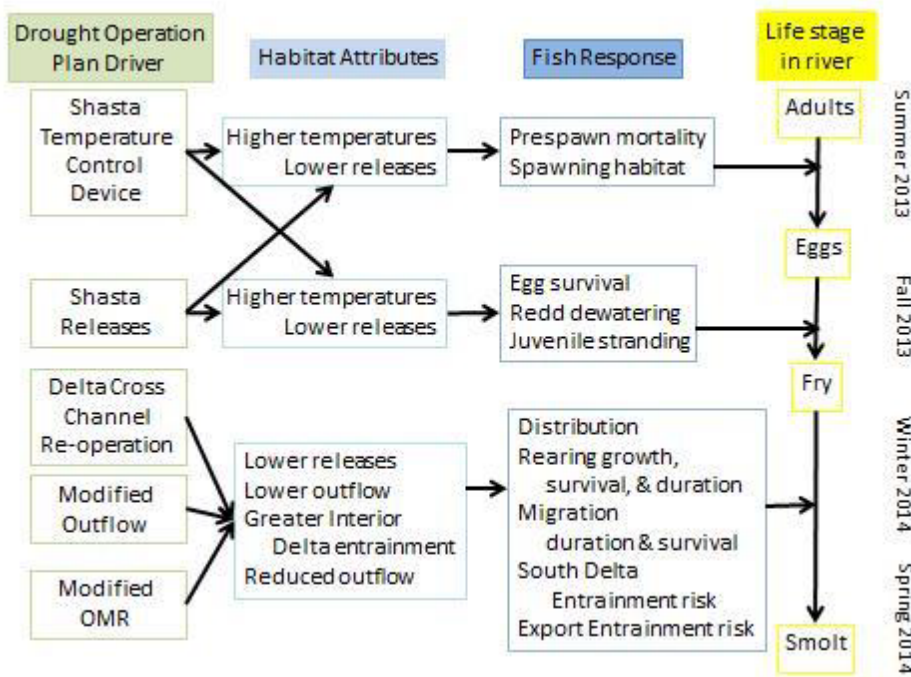
Figure 1. Conceptual model of salmon responses to drought actions from the Winter-Run Brood Year 2013 report (Israel et al. 2015).
